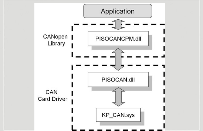
Library Structure
