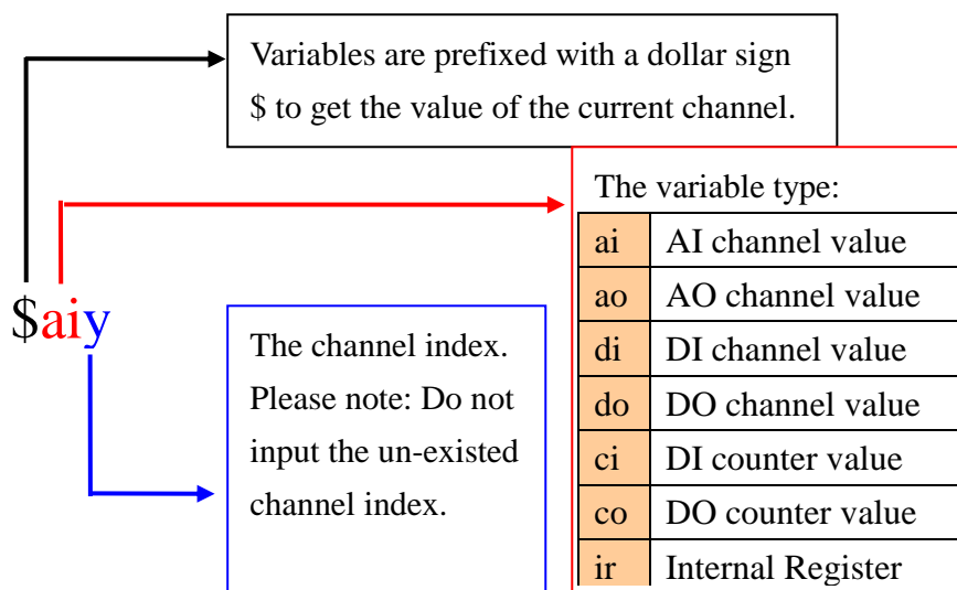
Figure 5-13 : Email channel value encoded syntax
