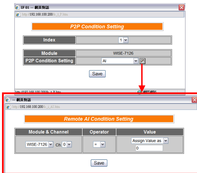
Figure 6-12 : P2P IF Condition detail setting page
