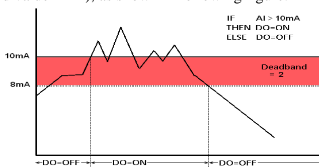
Figure 5-4 : AI Deadband Operation(> or >= a numerical value)
