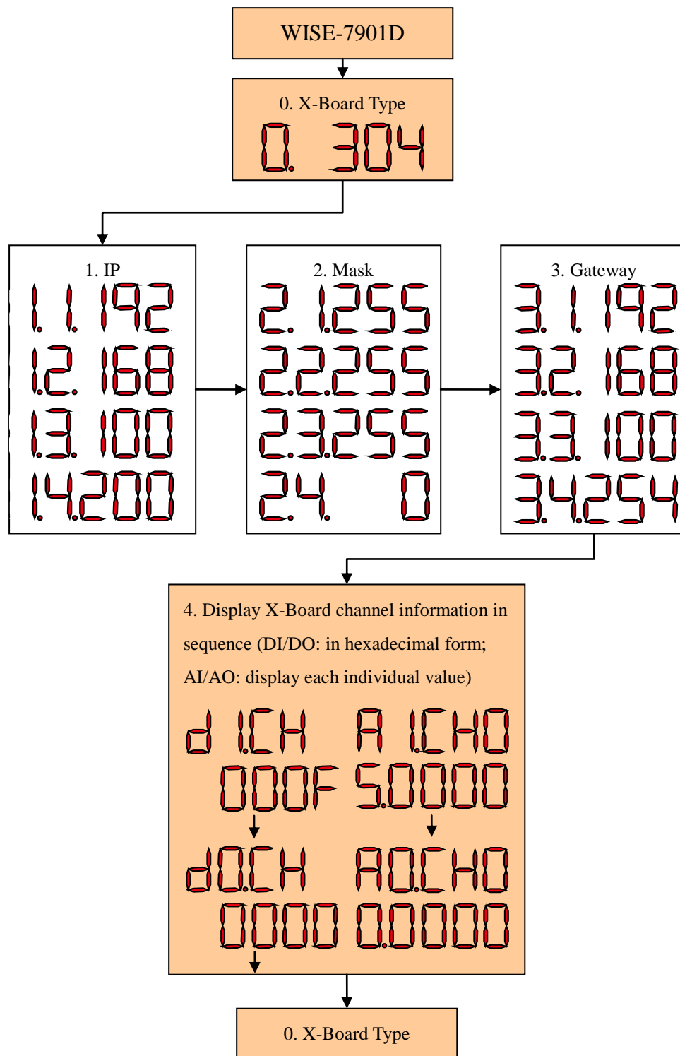
Figure 10-1 : The LED display shows network information and channel values
