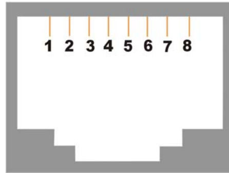
RJ-45
