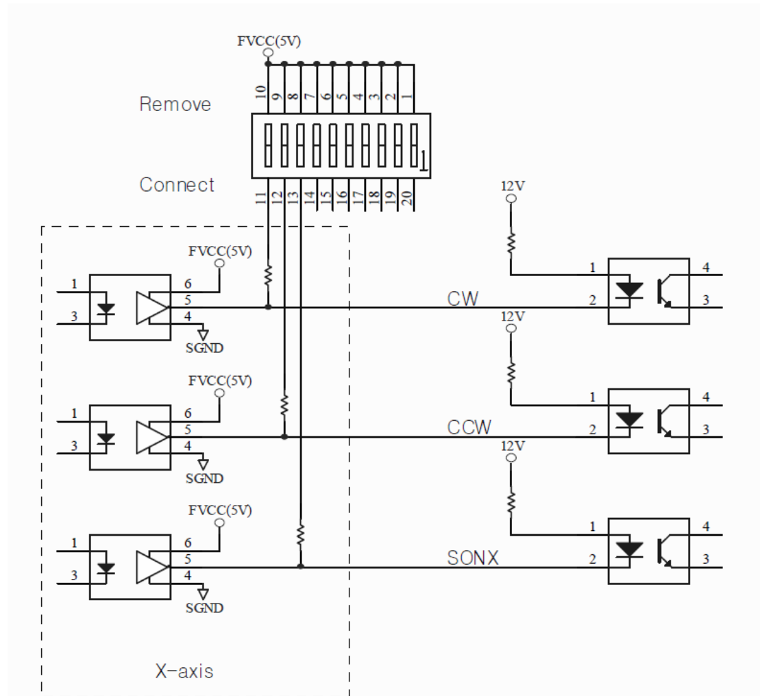
12 V motor driver connection
