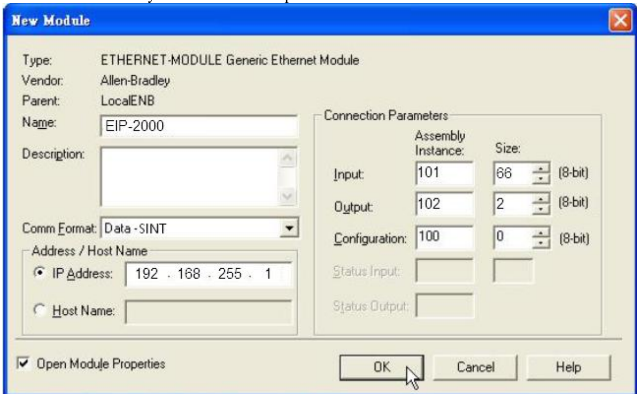
Figure5-5. The settings of EIP-2051 module
